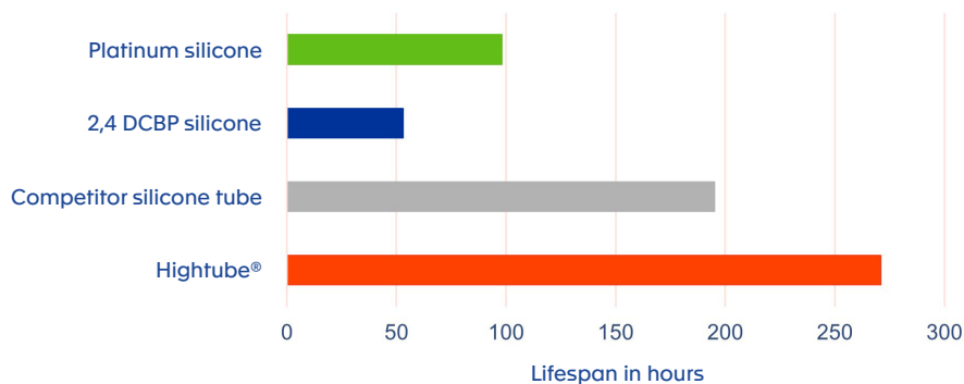
Lifespan on Ø4 × Ø6 tube 150 ml/min , 200 tr.min-1, 4-rollers pump
