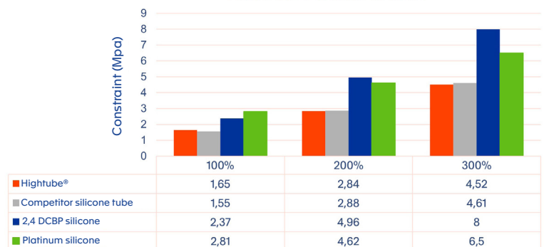
Secant modulus study
