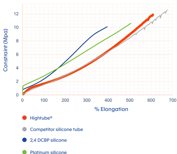
Tube tensil curve
